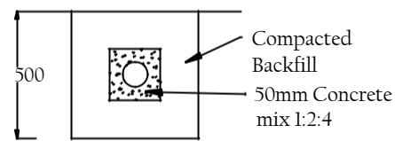
PIPE TRENCH
