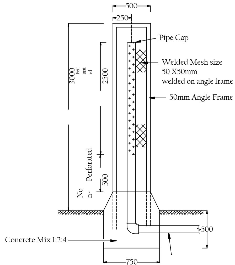
INTAKE TOWER
